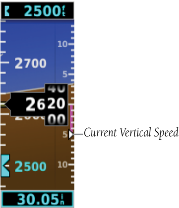
Figure 2-14 Vertical Speed Indicator
