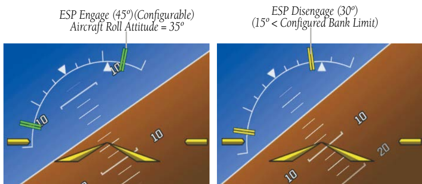
Figure 3-28 Roll Increasing to ESP Engagement
