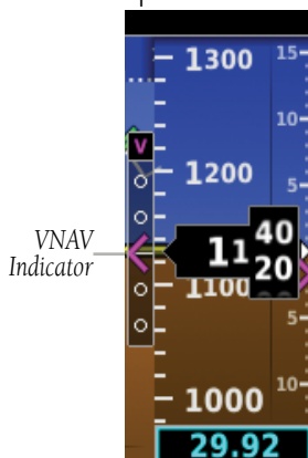
Figure 2-27 VNAV Indicator
